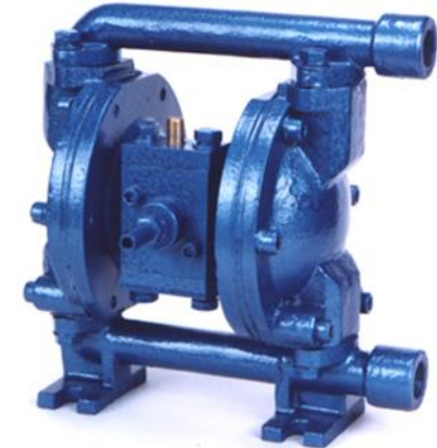
Air operated Double Diaphragm Pump
